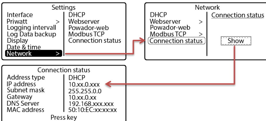
Figure 2. Access to remote config via the webserver menu interface on the inverter
