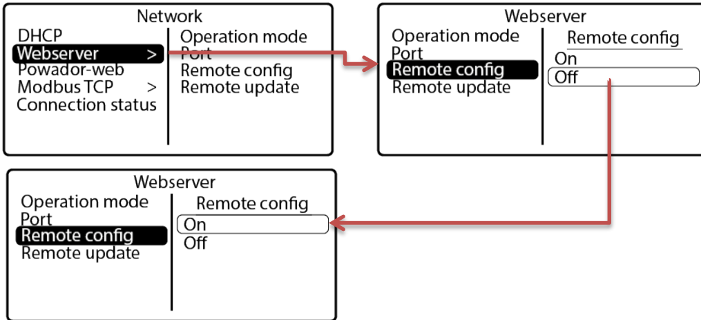
Figure 3. Access to remote config via the webservice menu interface on the inverter
