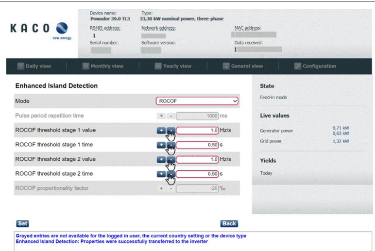
Figure 10. Enhanced Island Detection – Setting ROCOF
